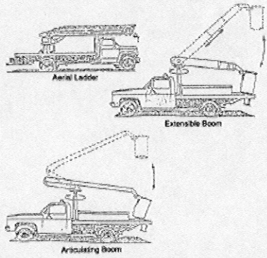
FIGURE 3 BOOM-SUPPORTED ELEVATING WORK PLATFORMS
