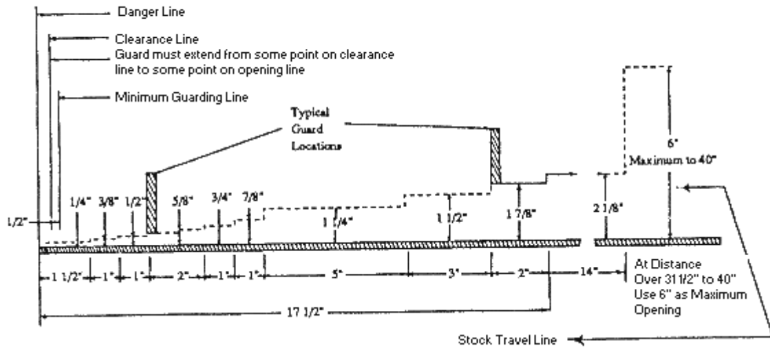
FIGURE 4 POSITIONING OF GUARD
