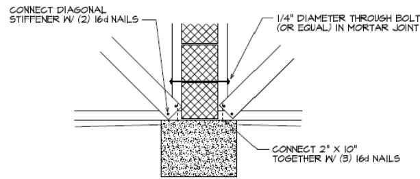
CONNECTION DETAIL
