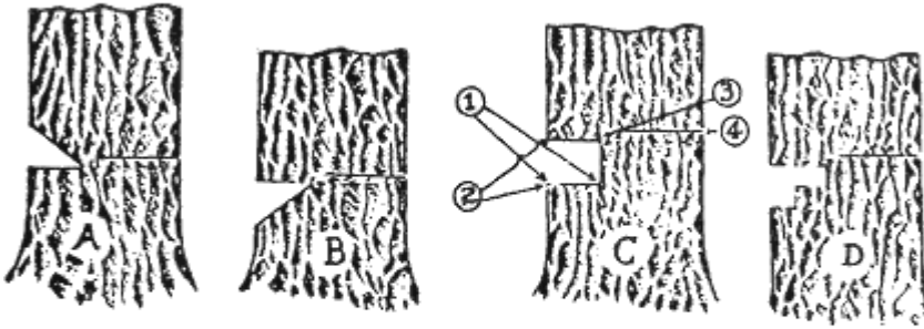
FIGURE 1 Approved Undercuts
